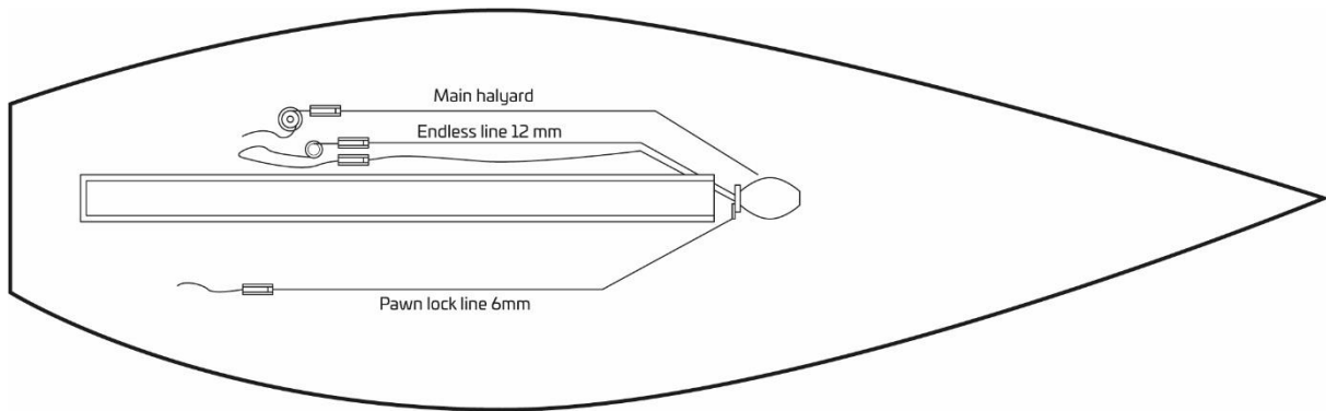
Layout with snubber winch (endless line in reefing position)
